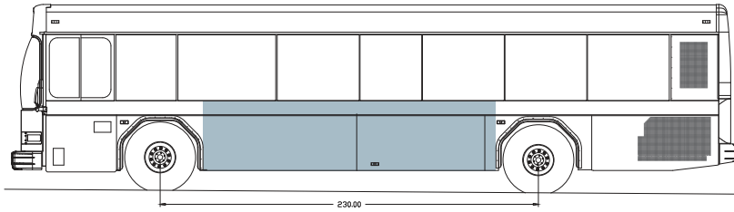
Driver Side Quarter Wrap 42" H x 178" W
